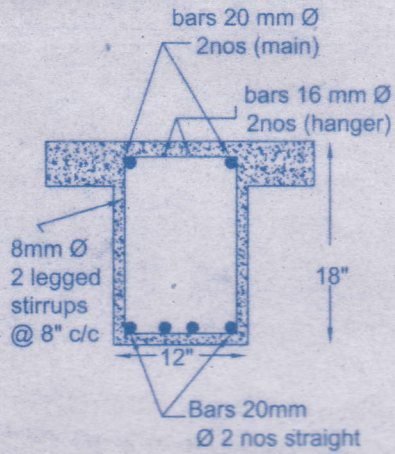
SECTION AT MIDDLE
