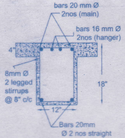
SECTION AT END
