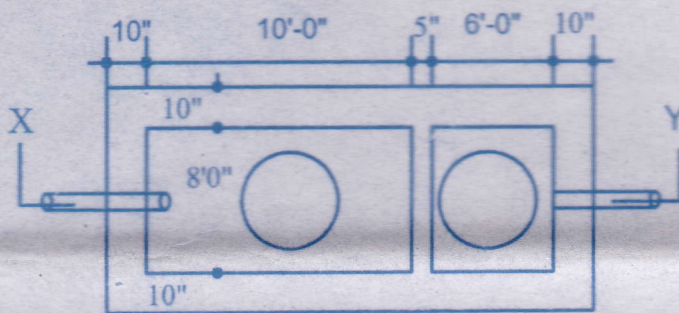
PROPOSED PLAN OF THE SEPTIC TANK
