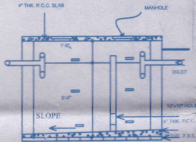
SECTION OF THE SEPTIC TANK
