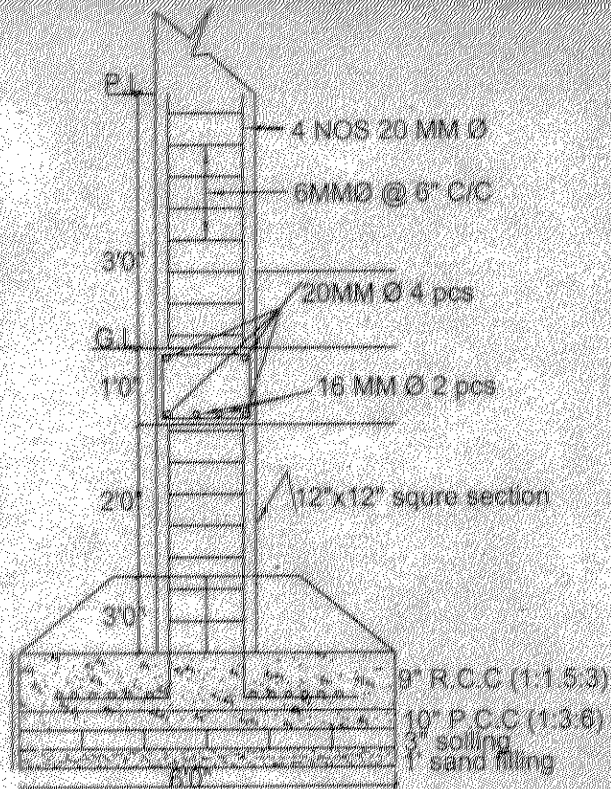
DETAILS OF COLUMN FOOTING (C1) SACLE :- 1"=4'0"
