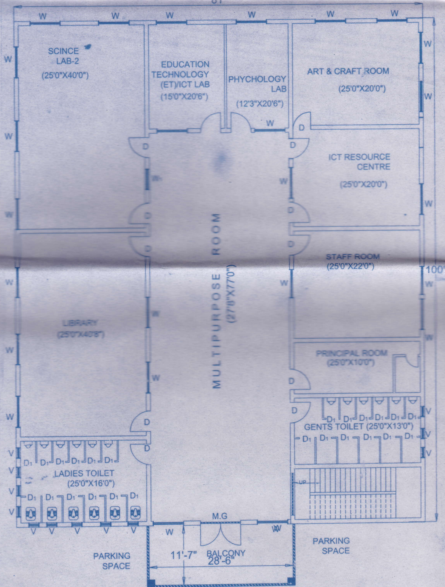
PROPOSED PLAN OF THE FIRST FLOOR
